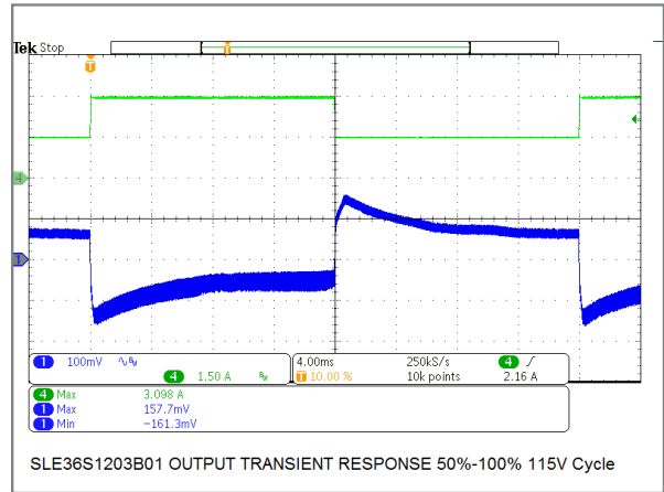
36W/12V Model Transient Response
