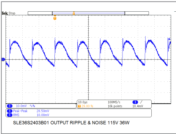
36W/24V Model Output Ripple & Noise at Full Load
