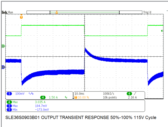
36W/9V Model Transient Response
