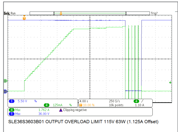
36W/36V Model Output Overload Protection
