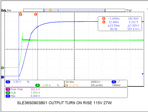
36W/9V Model Output Turn-On Rise Time
