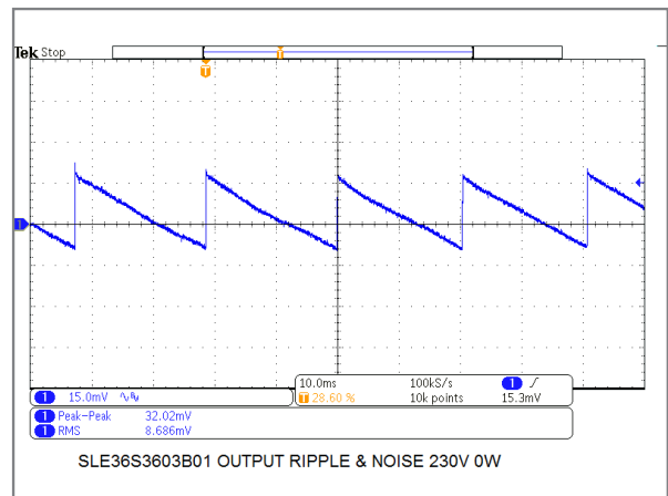
36W/36V Model Output Ripple & Noise at No Load
