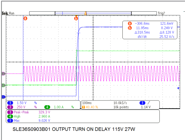
36W/9V Model Turn-On Delay Time
