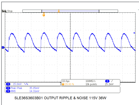
36W/36V Model Output Ripple & Noise at Full Load
