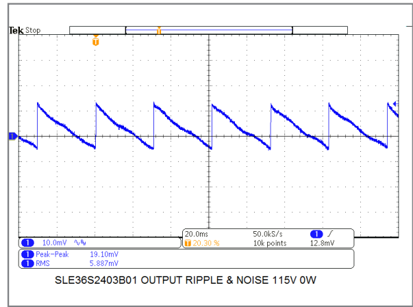
36W/24V Model Output Ripple & Noise at No Load
