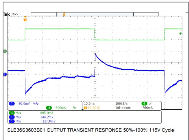
36W/36V Model Transient Response
