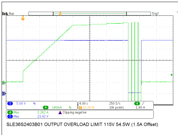
36W/24V Model Output Overload Protection
