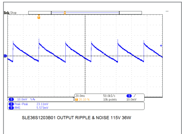
36W/12V Model Output Ripple & Noise at No Load
