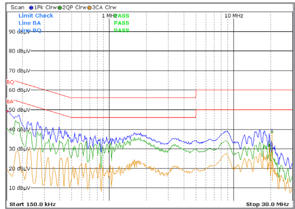
36W/9V Model _ Neutral 120V/60Hz 100% 9V@3.0A
