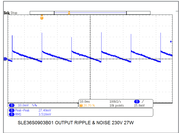
36W/9V Model Output Ripple & Noise at No Load
