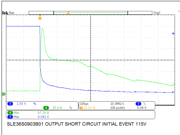
36W/9V Model Output Short Circuit Initial Event
