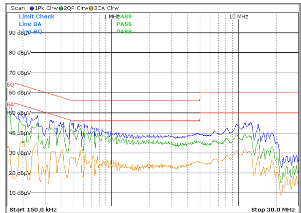
36W/12V Model _ Neutral 120V/60Hz 100% 12V@3A
