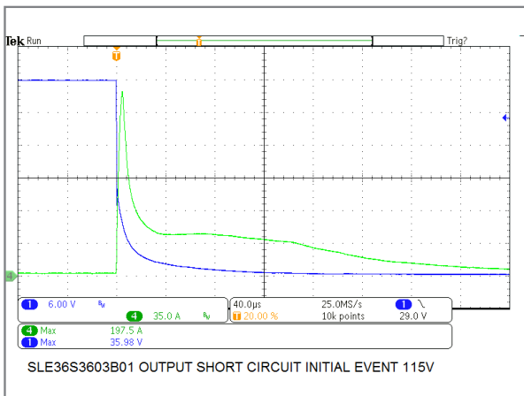
36W/36V Model Output Short Circuit Initial Event
