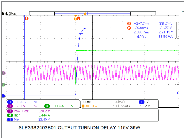
36W/24V Model Turn-On Delay Time
