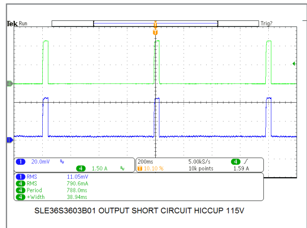
36W/36V Model Output Short Circuit Hiccup Mode
