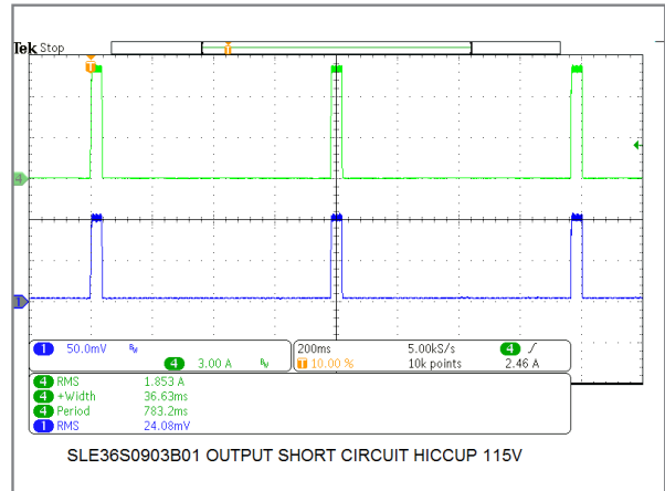
36W/9V Model Output Short Circuit Hiccup Mode
