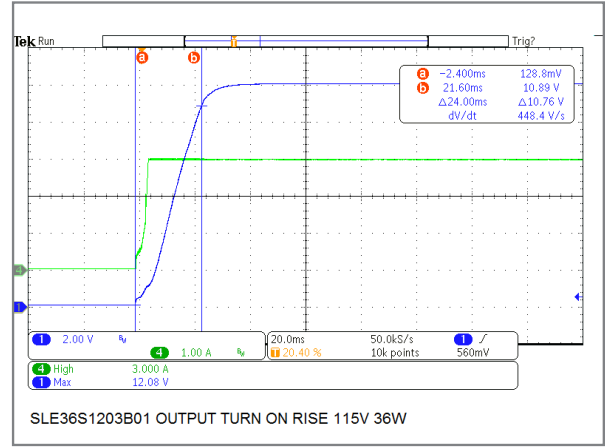
36W/12V Model Output Turn-On Rise Time
