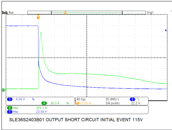
36W/24V Model Output Short Circuit Initial Event
