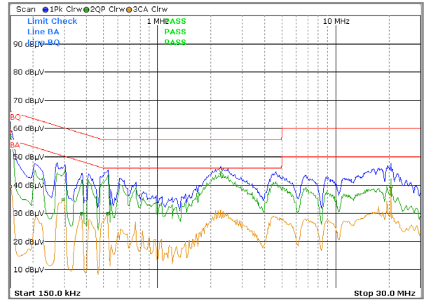
36W/24V Model _ Neutral 120V/60Hz 100% 24V@1.5A
