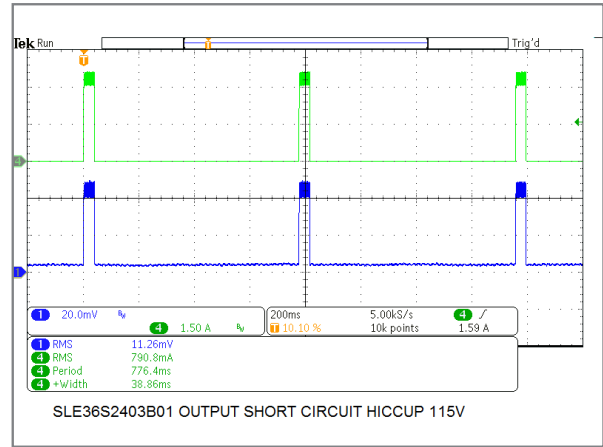
36W/24V Model Output Short Circuit Hiccup Mode
