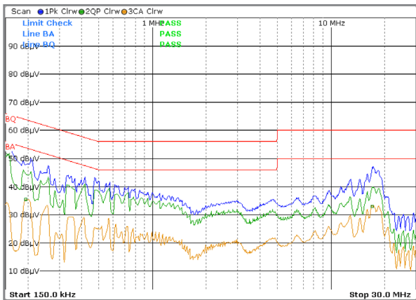
36W/12V Model _ Line 120V/60Hz 100% 12V@3A
