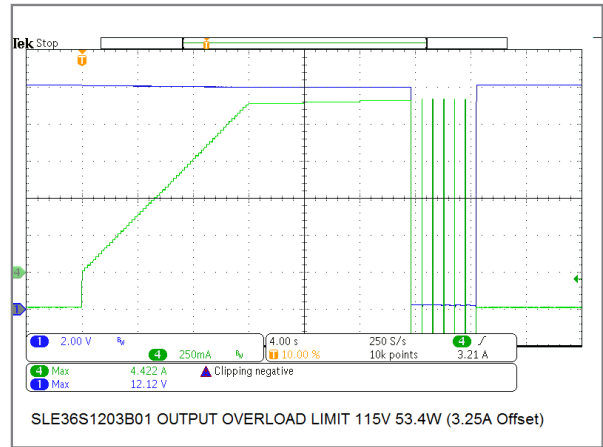
36W/12V Model Output Overload Protection
