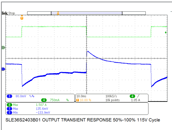
36W/24V Model Transient Response
