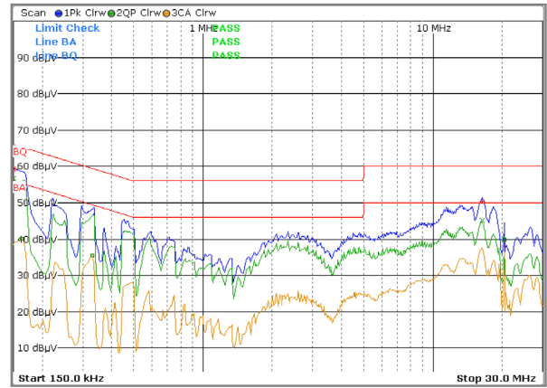
36W/36V Model _ Neutral 120V/60Hz 100% 36V@1.0A
