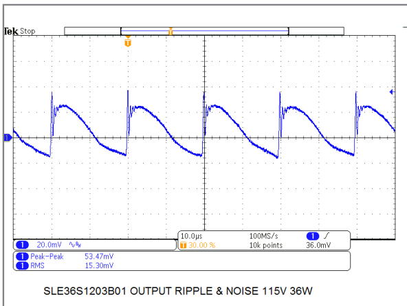
36W12V Model Output Ripple & Noise at Full Load
