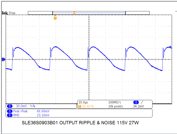
36W/9V Model Output Ripple & Noise at Full Load
