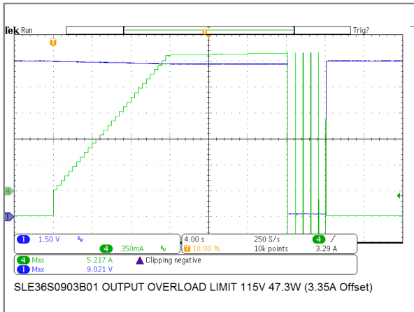
36W/9V Model Output Overload Protection
