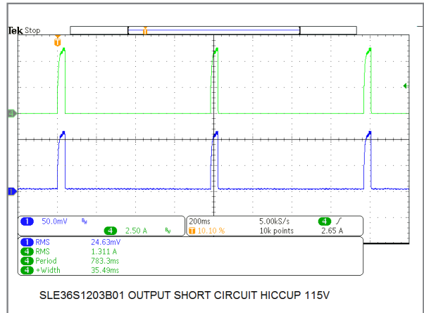
36W/12V Model Output Short Circuit Hiccup Mode
