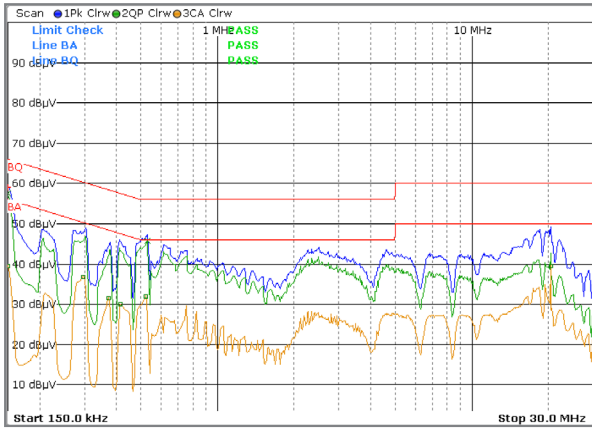
36W/24V Model _ Line 120V/60Hz 100% 24V@1.5A
