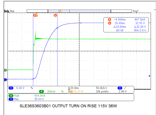
36W/36V Model Output Turn-On Rise Time
