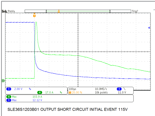
36W/12V Model Output Short Circuit Initial Event
