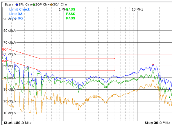
36W/36V Model _ Line 120V/60Hz 100% 36V@1.0A
