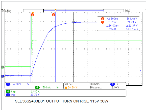
36W/24V Model Output Turn-On Rise Time
