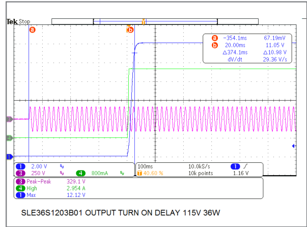
36W/12V Model Turn-On Delay Time
