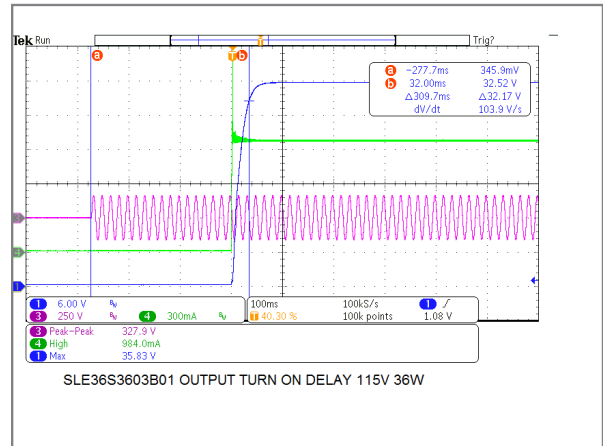
36W/36V Model Turn-On Delay Time
